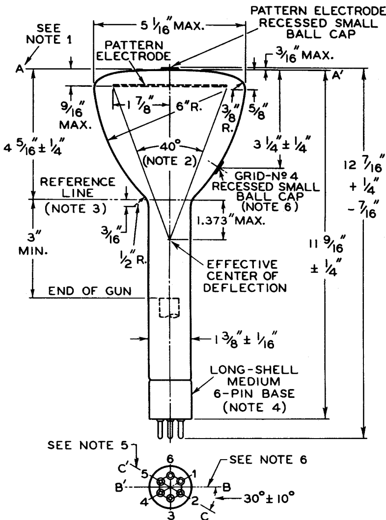
BOTTOM VIEW
